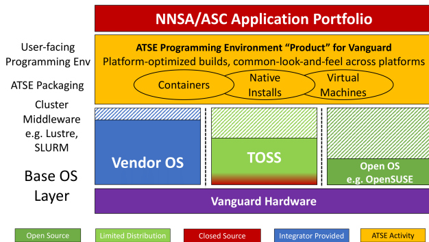
Figure 1: ATSE provides a common environment over a variety of operating systems.
