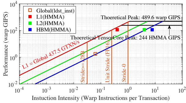
(a) Visualized global memory pattern of cudaTensorCoreGemm in Instruction Roofline on GV100.
