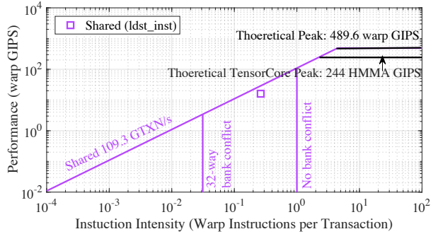
(b) Visualized shared memory pattern in Instruction Roofline on GV100.
