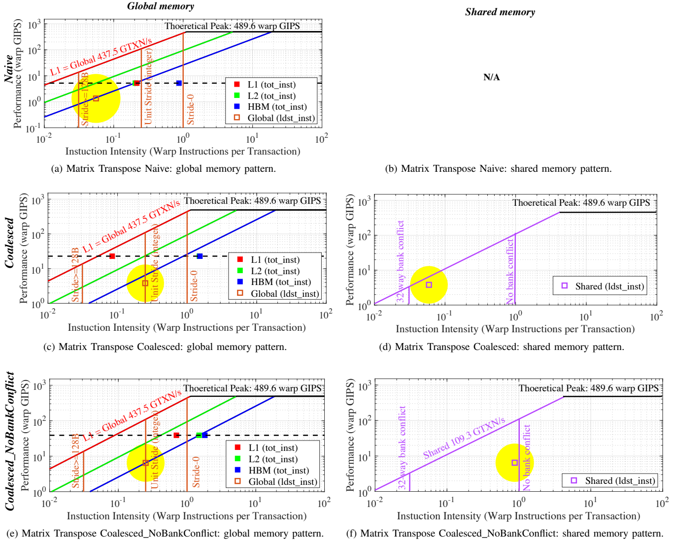
Figure 7: Instruction Roofline on GV100 for the three implementations in Matrix Transpose. The solid dots are the total number of instructions (tot_inst) executed by non-predicated threads. The open dots refer to memory access patterns.
